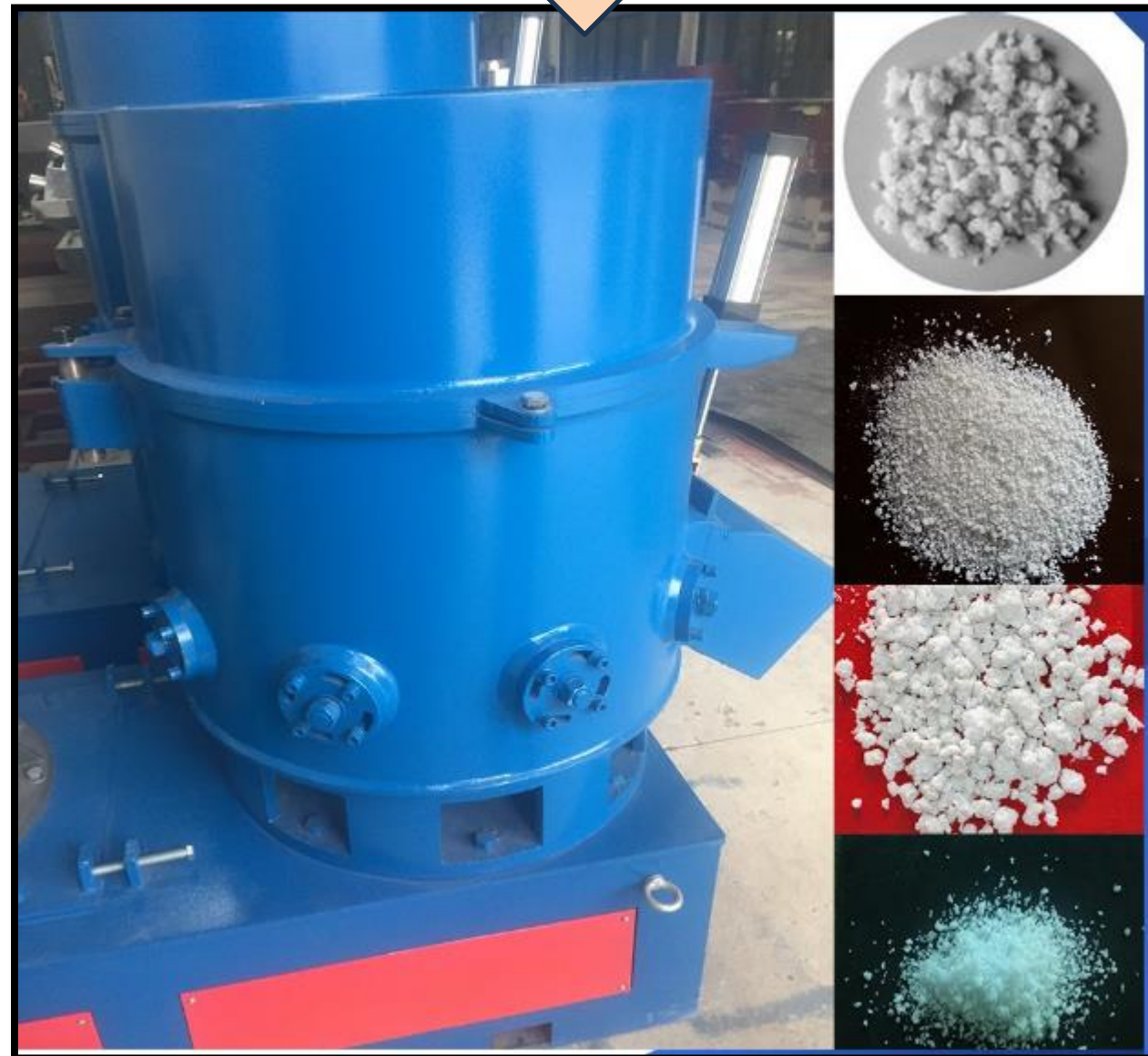
AGGLOMORATER MACHINE
